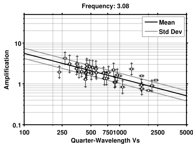
Figure 4. Correlation between quarter-wavelength average velocities and amplification factors from spectral modeling of earthquake spectra. A linear least-squares regression is applied in log-log scale to estimate parameter correlation.
