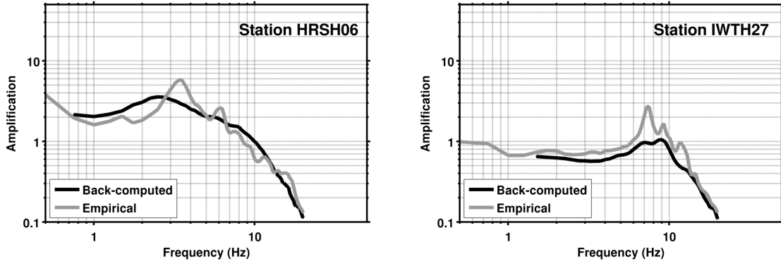
Figure 8. Comparison between empirical and back-computed amplification functions at two example KiK-Net test sites using the coefficients from the frequency dependent correlations.
