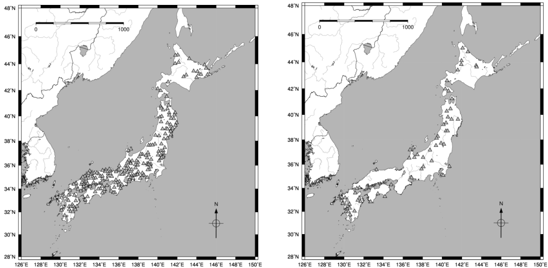
Figure 2. Location of the selected sites of the Japanese KiKNet network. On the left the 220 soft sediment sites, and on the right the 59 stiff-soil and rock sites.
