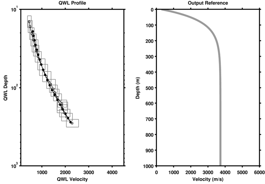
Figure 5. On the left, quarter-wavelength representation of the reference velocity profile obtained from the correlations between quarter-wavelength average velocities and amplification factors. On the right, the inverted reference velocity profile in standard representation.
