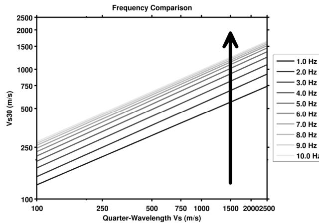
Figure 12. Comparison between all the V_{S_{30}}-V_{S^{Qwl}} regressions performed in the frequency range 1-10Hz. While regression slopes are basically constant, intercepts smoothly increases with increasing frequencies.
