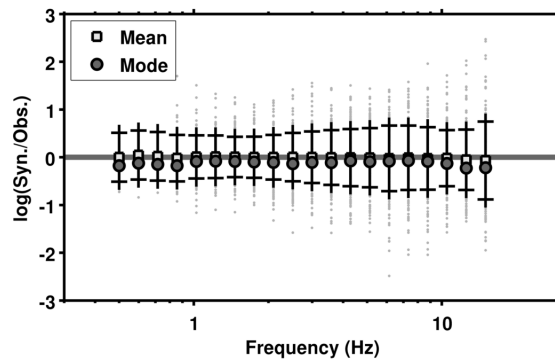
Figure 9. Distribution of the residuals between observed (empirical) and computed amplification functions over the analyzed frequency range (0.5-20Hz).
