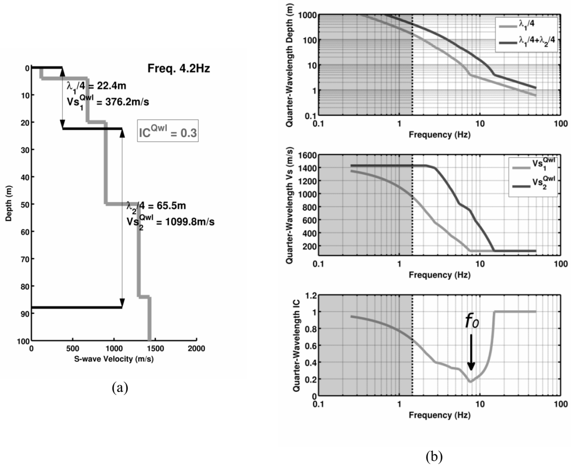
Figure 1. Example of quarter-wavelength depth ( \lambda/4 ), velocity ( V_S^{Qwl} ) and seismic impedance contrast ( IC^{Qwl} ) curves (b) of a shear-wave velocity profile (a). The black dashed line defines the frequency region of reliability, where the curves are constrained by the measured velocity profile.
