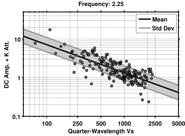
Figure 6. Frequency dependent relation between the damped site term A^{DC}A^k with the quarter-wavelength average velocity at the different sites. Here and example at 2.25Hz.
