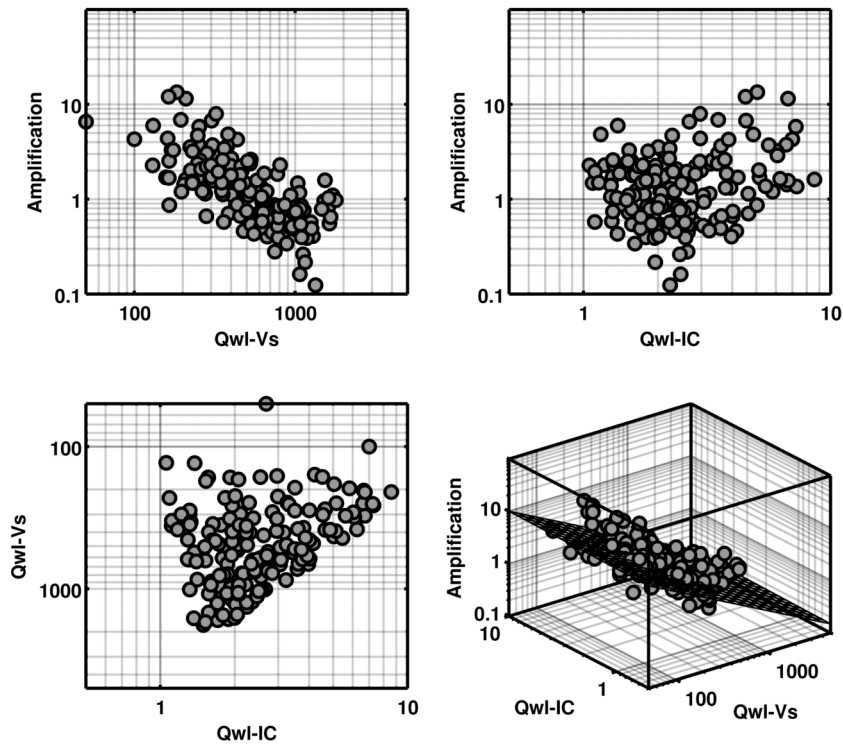
Figure 7. Correlation between the empirical amplification from spectral modeling, the \frac{1}{4} wavelength-Vs ( V_s^{Qwl} ) and the \frac{1}{4} wavelength-IC ( IC^{Qwl} ) parameters. For the regression, the 220 selected sites of the Japanese network were used. Each dot corresponds to one site. The plots are for a frequency of 3.5Hz.
