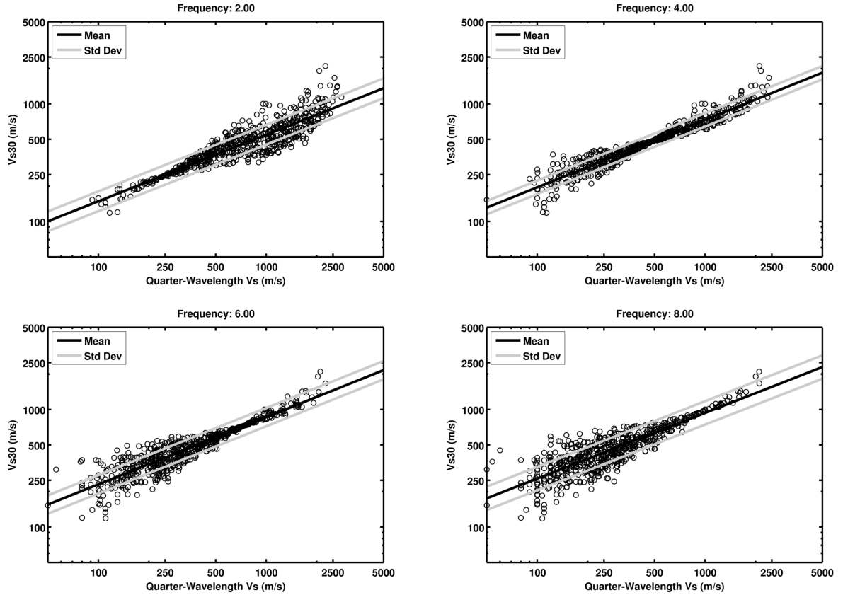
Figure 11. Example of correlation between V_{S30} and V_S^{Qwl} at four discrete frequencies (2, 4, 6 and 8Hz). Each dot represents a station.
